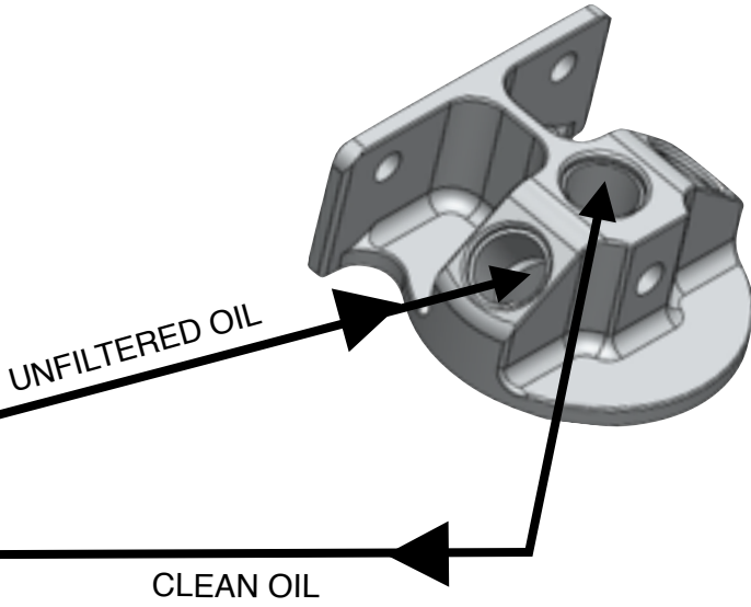
NO OIL COOLER DETAIL
